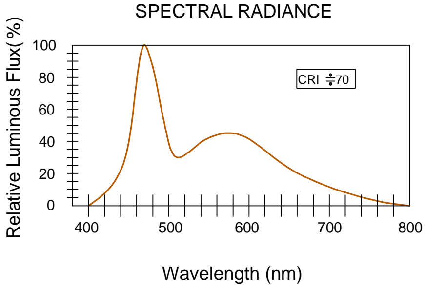
Fig.5 Luminous Spectrum(Ta=25 )
