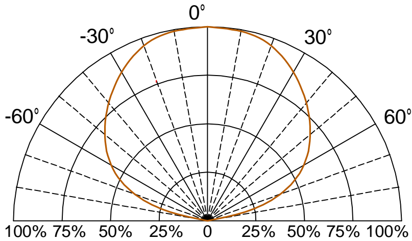
Fig.6 Directivity Radiation
