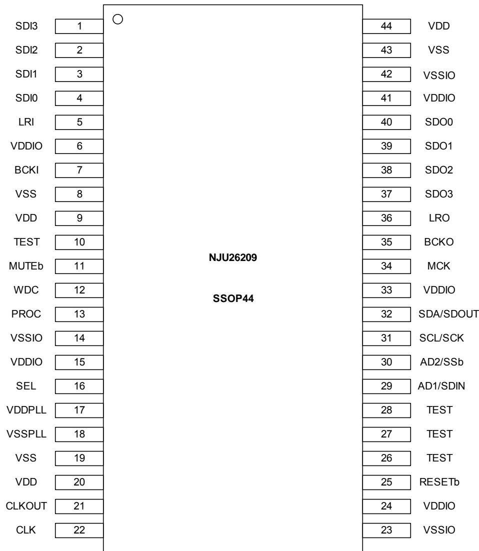
Fig. 3 NJU26209 Pin Configuration
