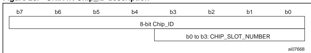
Figure 20. SRIX4K Chip_ID description
