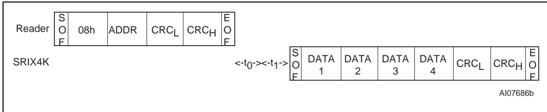
Figure 61. READ_BLOCK frame exchange between Reader and SRIX4K
