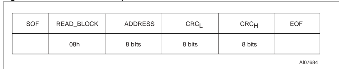
Figure 41. READ_BLOCK request format
