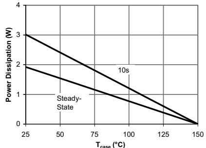
Figure 13: Power De-rating (Note A)
