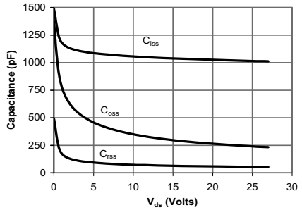
Figure 8: Capacitance Characteristics
