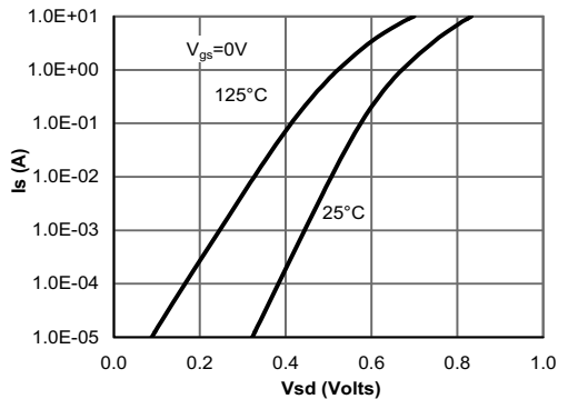
Figure 6: Body-Diode Characteristics
