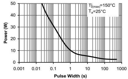
Figure 10: Single Pulse Power Rating Junction-to-Ambient (Note E)
