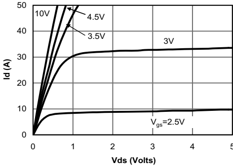
Fig 1: On-Region Characteristics
