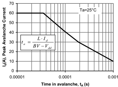
Figure 12: Avalanche capability
