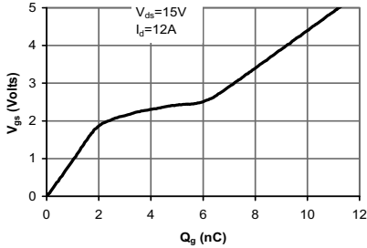
Figure 7: Gate-Charge Characteristics
