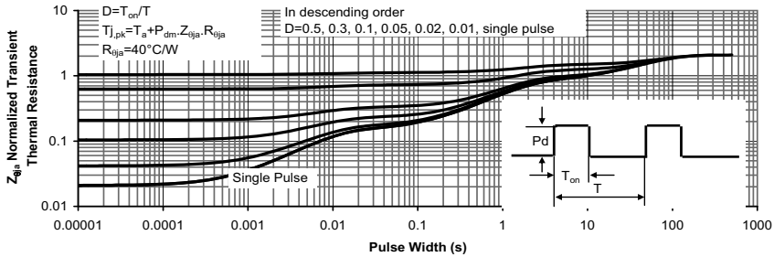
Figure 11: Normalized Maximum Transient Thermal Impedance
