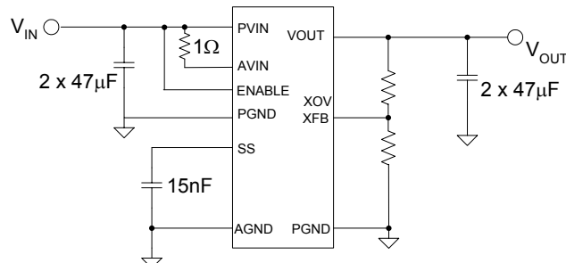
Figure 1. Simple Layout.
