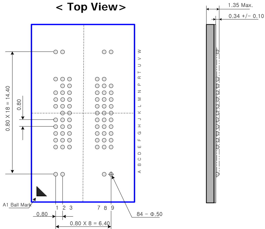
< Bottom View >
