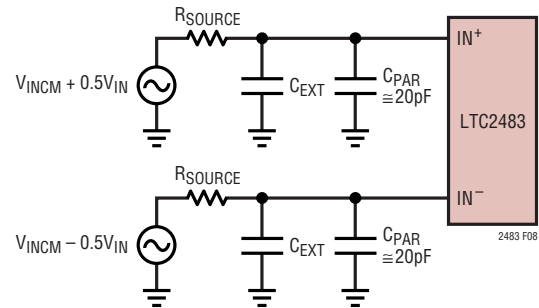
Figure 8. An RC Network at IN + and IN -
