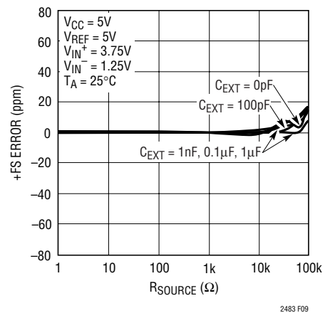
Figure 9. +FS Error vs R_{\text{SOURCE}} at IN + and IN -
