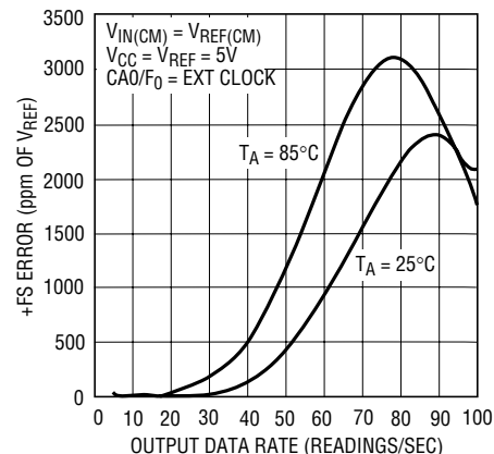
Figure 17. +FS Error vs Output Data Rate and Temperature
