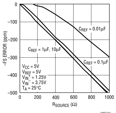
Figure 14. -FS Error vs R_{SOURCE} at REF^+ or REF^- (Large C_{REF} )
