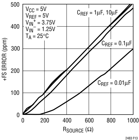
Figure 13. +FS Error vs R_{SOURCE} at REF^+ or REF^- (Large C_{REF} )
