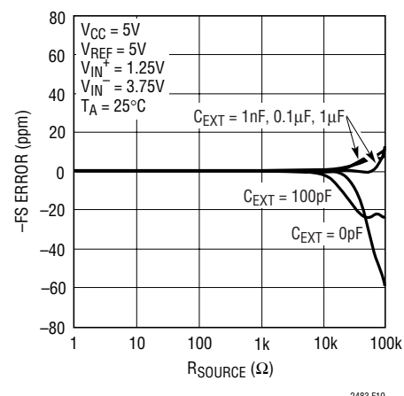
Figure 10. -FS Error vs R_{\text{SOURCE}} at IN + and IN -
