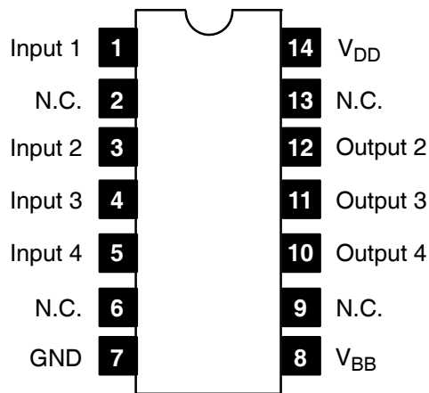
Pin Connection Diagram
