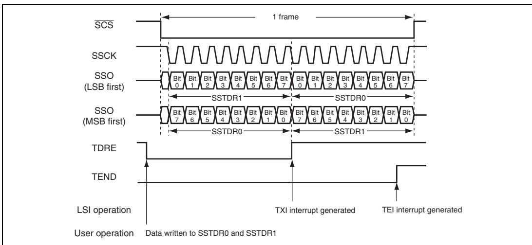
Figure 15.5 Example of Transmission Operation (SSU Mode) (2) When 16-bit data length is selected (SSTD0 and SSTD1 are valid) with CPOS = 0 and CPHS = 0
