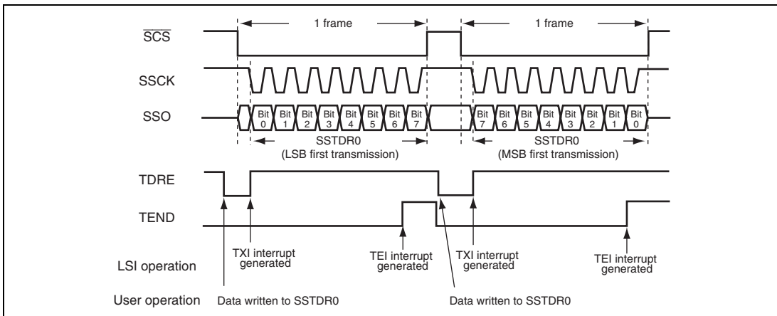
Figure 15.5 Example of Transmission Operation (SSU Mode) (1) When 8-bit data length is selected (SSTD0 is valid) with CPOS = 0 and CPHS = 0
