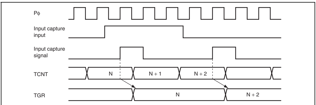
Figure 9.33 Input Capture Input Signal Timing
