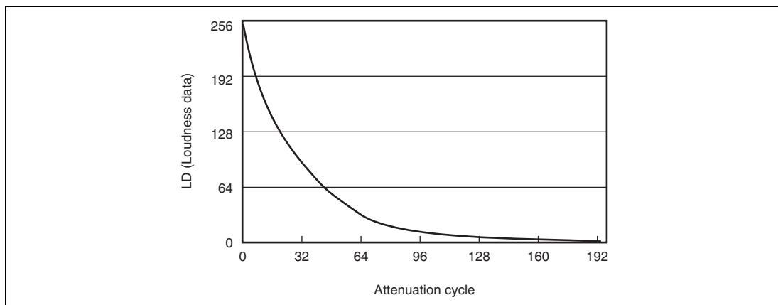
Figure 20.4 Attenuation Characteristics
