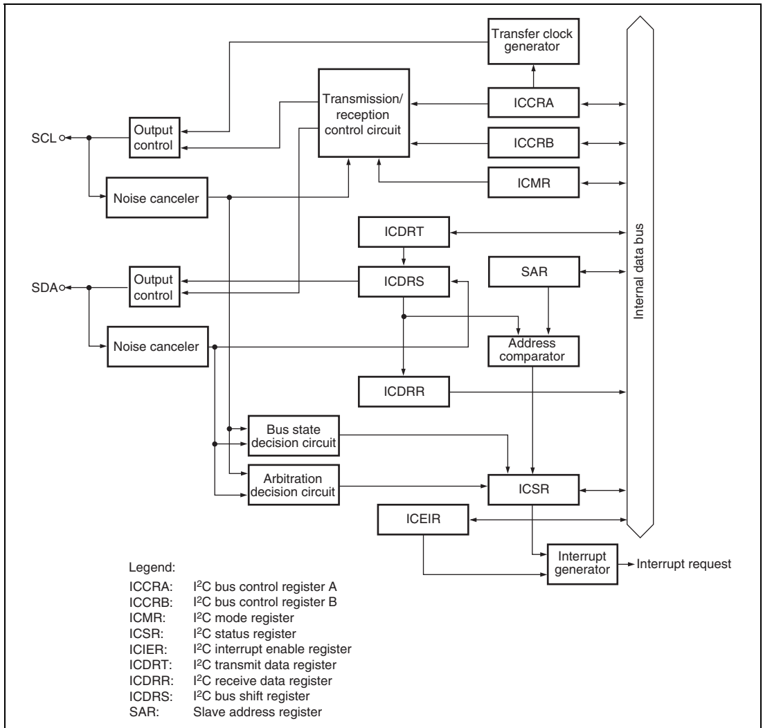
Figure 13.1 Block Diagram of I 2 C Bus Interface 2
