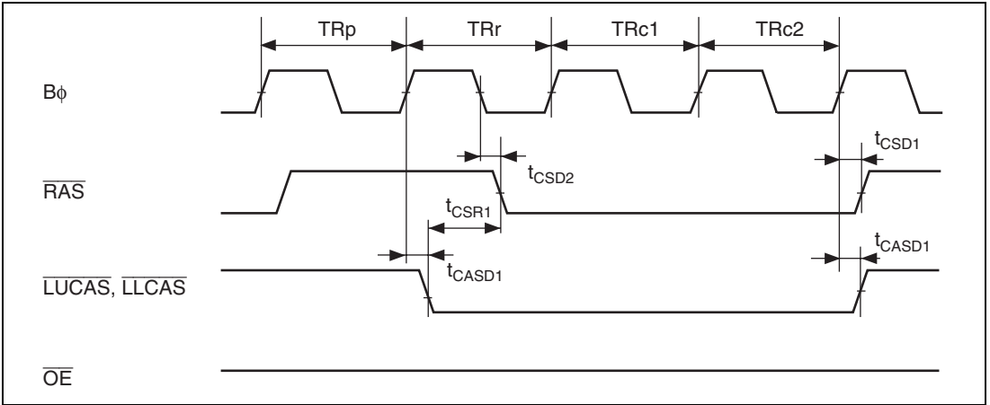
Figure 29.25 CAS before RAS Refresh Timing*
