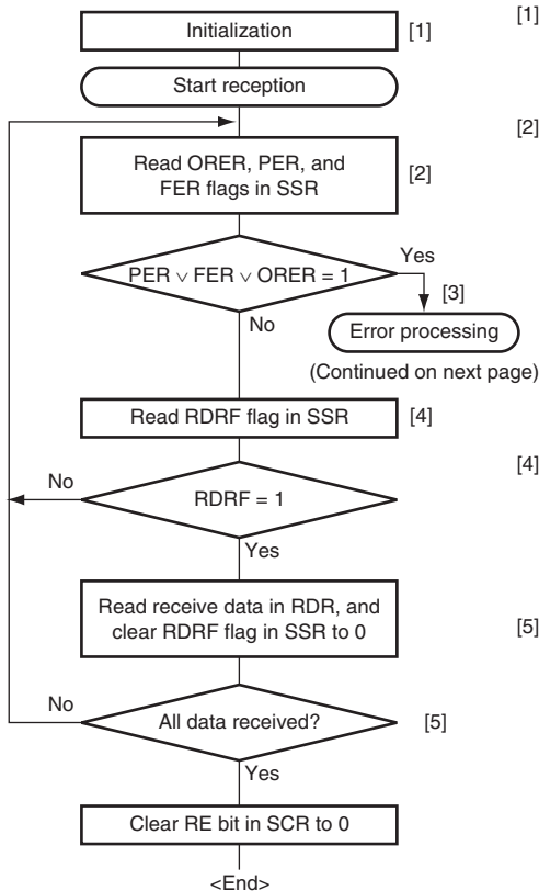
Figure 19.12 Sample Serial Reception Flowchart (1)
