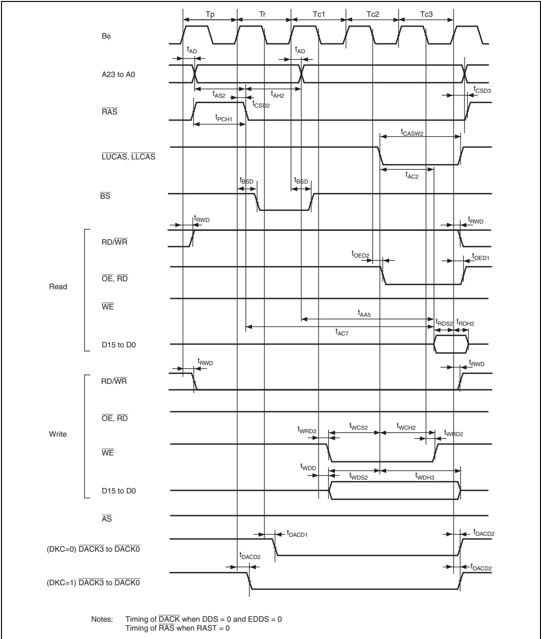
Figure 29.22 DRAM Access Timing / Three-State Access (When RAST=1)*
