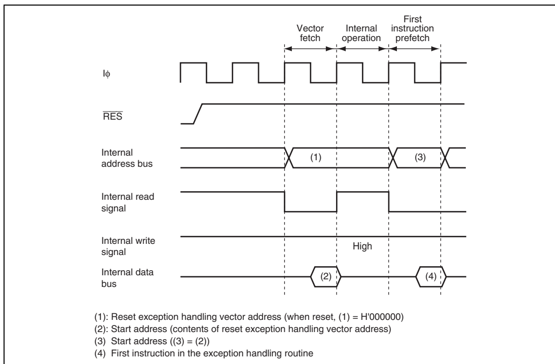
Figure 6.1 Reset Sequence (On-chip ROM Enabled Advanced Mode)
