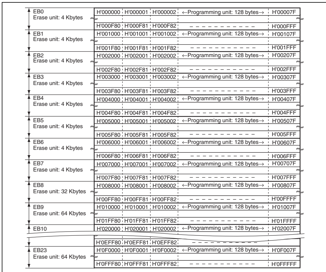
Figure 24.4 User MAT Block Structure of H8SX/1648
