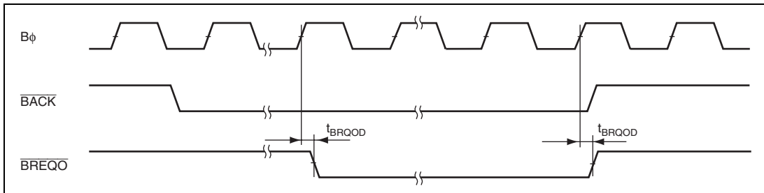
Figure 29.36 External Bus Request Output Timing
