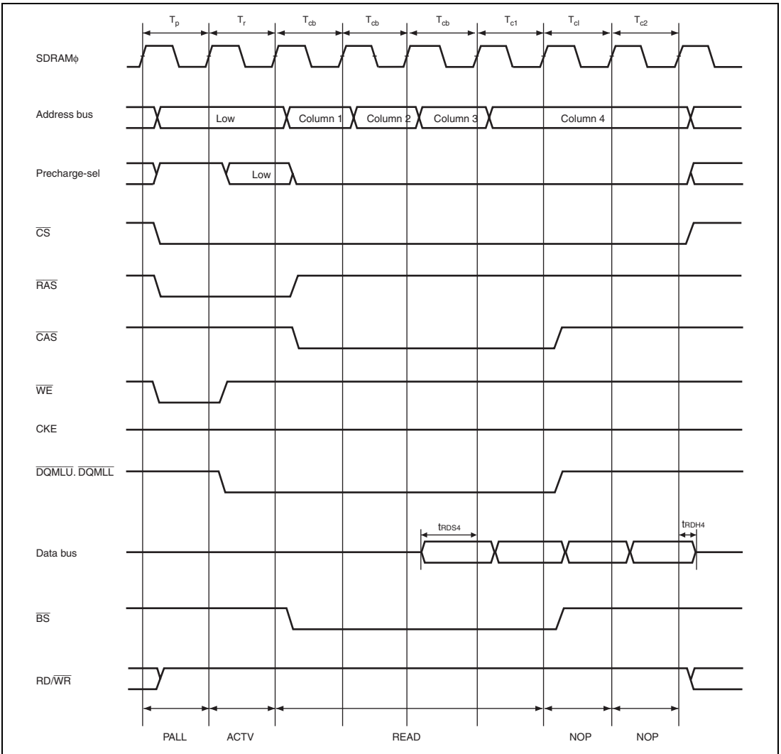
Figure 29.32 Synchronous DRAM Cluster Transfer Access Timing (Read)*
