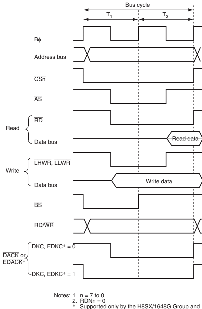
Figure 9.24 \overline{\text{DACK}} and \overline{\text{EDACK}}^* Signal Output Timing
