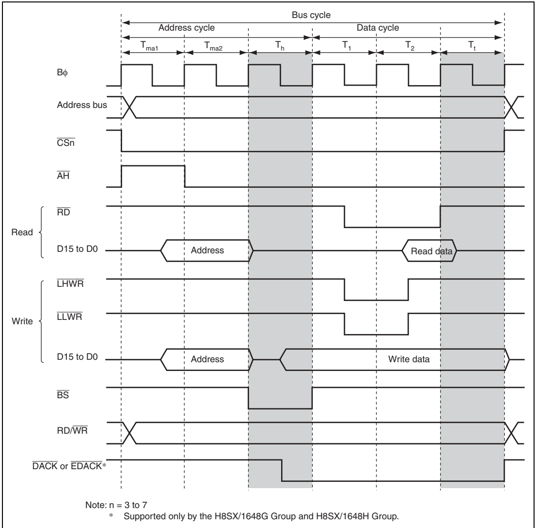
Figure 9.35 Chip Select ( \overline{CS} ) Assertion Period Extension Timing in Data Cycle
