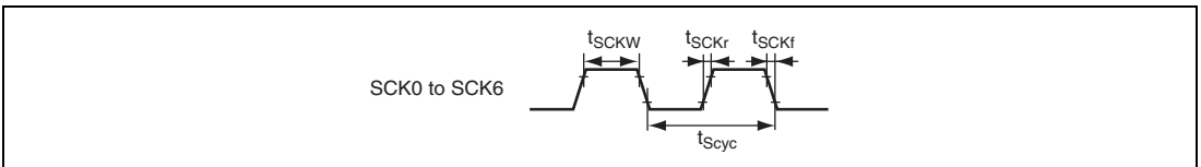
Figure 29.50 SCK Clock Input Timing
