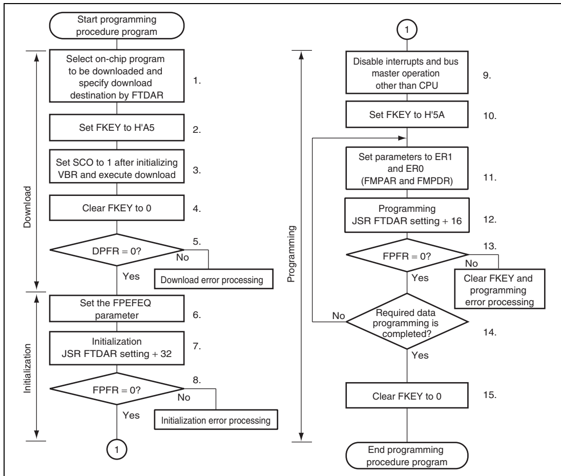
Figure 24.11 Programming Procedure in User Program Mode
