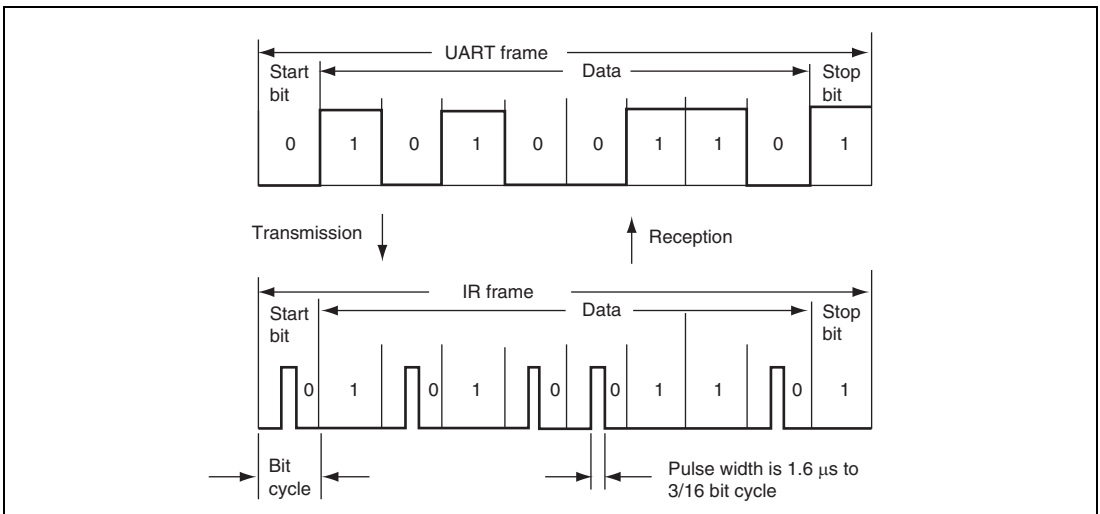
Figure 19.37 IrDA Transmission and Reception
