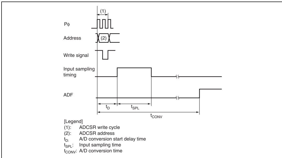
Figure 21.7 A/D Conversion Timing
