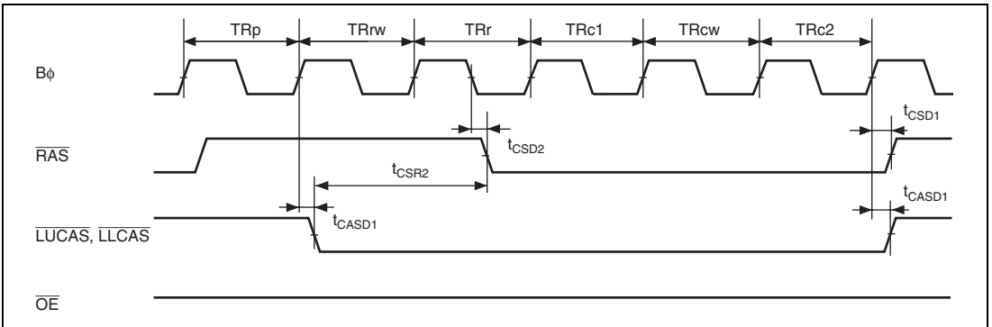
Figure 29.26 CAS before RAS Refresh Timing (Wait Cycle Inserted)*
