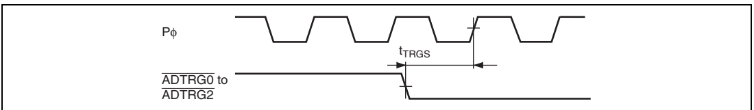
Figure 29.52 A/D Converter External Trigger Input Timing
