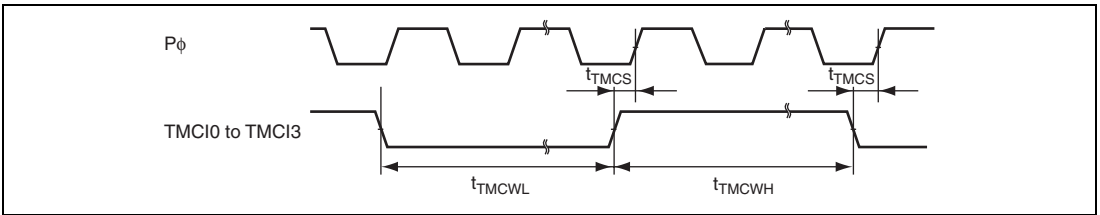
Figure 29.48 8-Bit Timer Clock Input Timing
