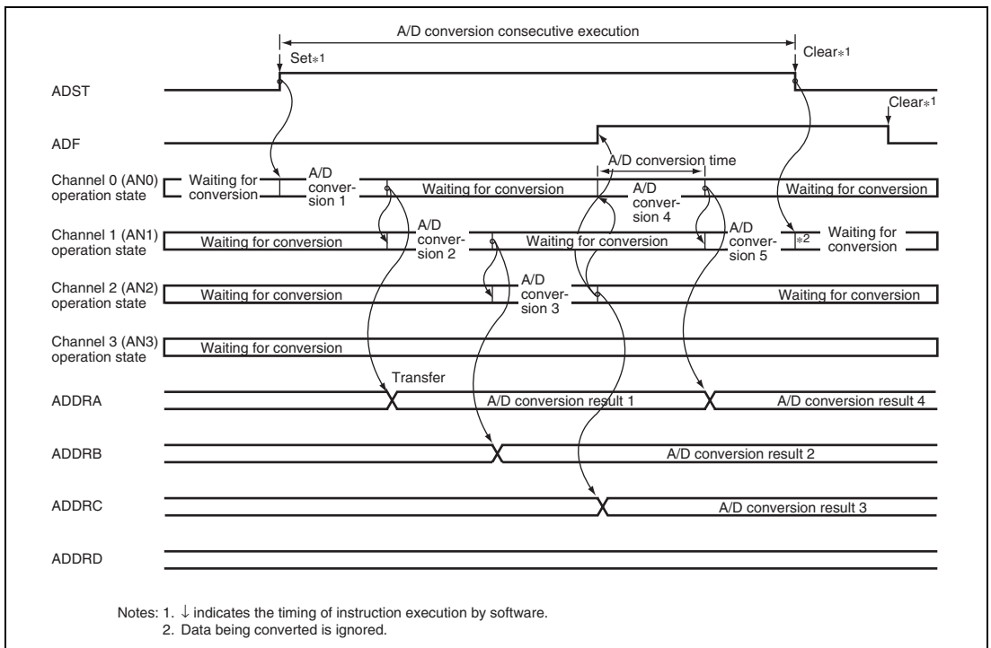
Figure 21.5 Example of A/D Conversion (Continuous Scan Mode, Three Channels (AN0 to AN2) Selected)
