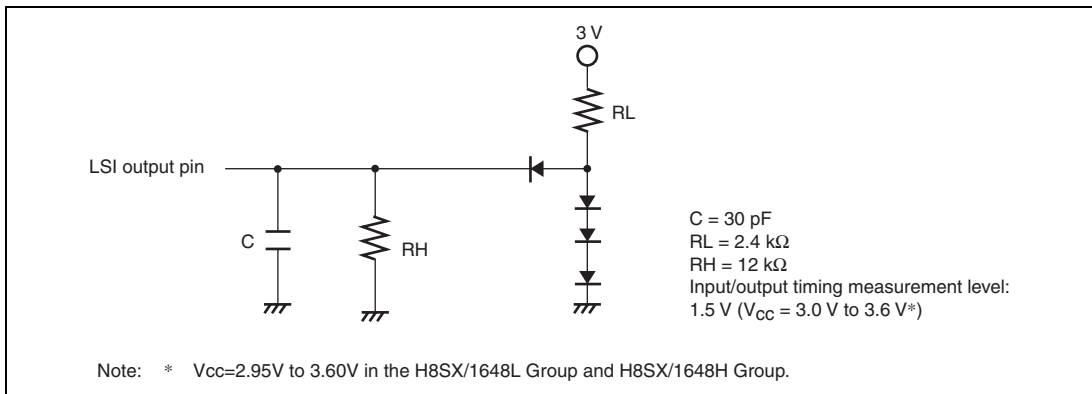
Figure 29.1 Output Load Circuit
