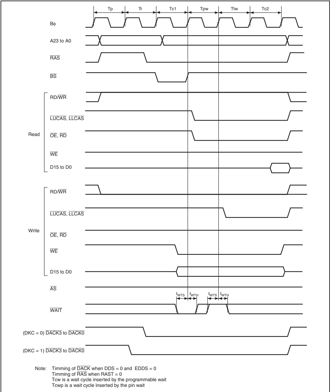
Figure 29.20 DRAM Access Timing / Two-State Access, One Wait*
