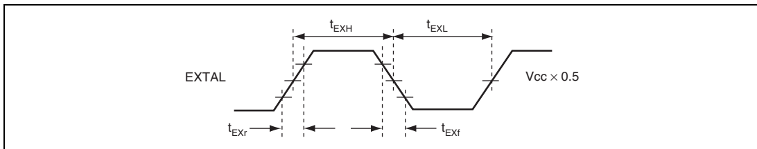
Figure 26.5 External Clock Input Timing
