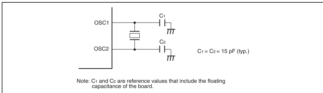
Figure 26.6 Connection Example of 32.768-kHz Crystal Resonator
