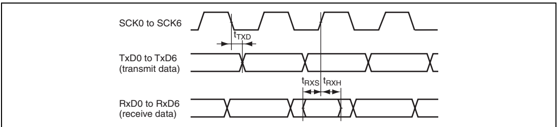
Figure 29.51 SCI Input/Output Timing: Clocked Synchronous Mode
