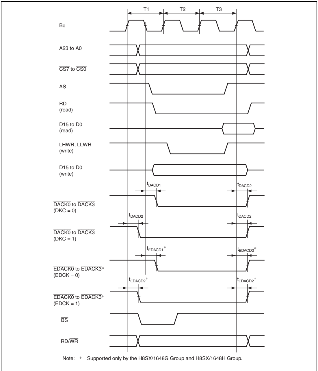
Figure 29.40 Single Address Transfer Timing for the DMAC and EXDMAC* (Three-State Access)
