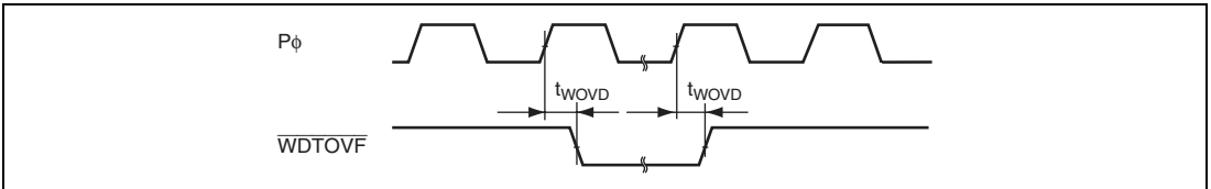
Figure 29.49 WDT Output Timing
