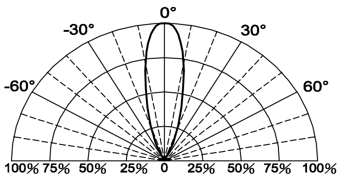
Fig.6 Directivity Radiation
