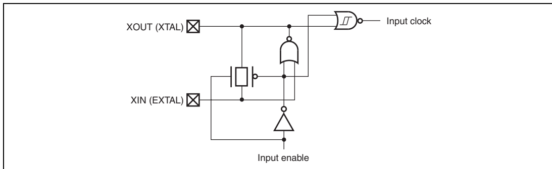
Figure 1.3 Simplified Circuit Diagram (Oscillation Buffer)
