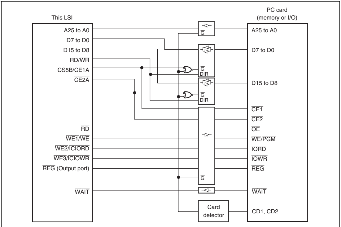
Figure 8.42 Example of PCMCIA Interface Connection
