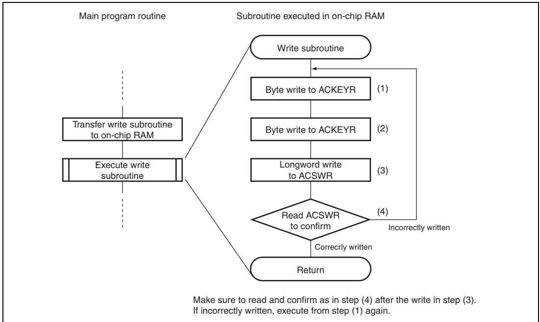
Figure 8.2 Recommended Sequence to Write to ACSWR
