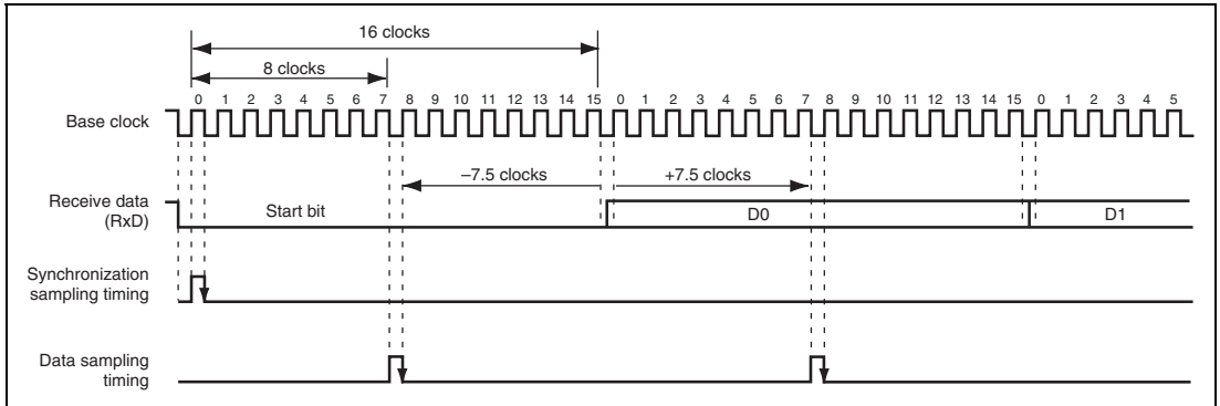
Figure 15.19 Receive Data Sampling Timing in Asynchronous Mode
