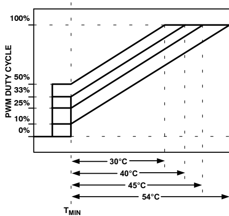
Figure 59. Increasing PWM_{MIN} Changes Effective T_{RANGE}
