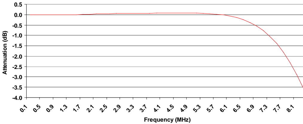
Figure 4. FMS6646 SD Frequency Response (Flatness)
