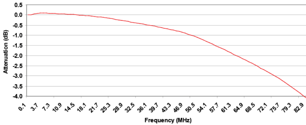
Figure 6. FMS6646 HD Frequency Response (Flatness)
