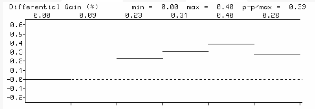
Figure 7. Differential Gain
