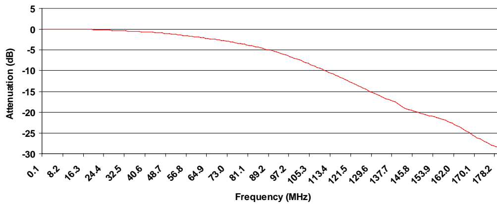
Figure 5. FMS6646 HD Frequency Response
