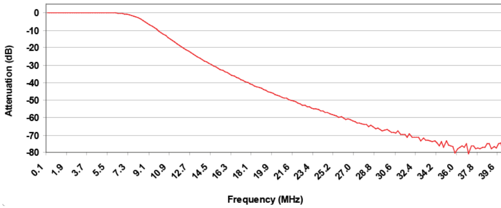
Figure 3. FMS6646 SD Frequency Response
