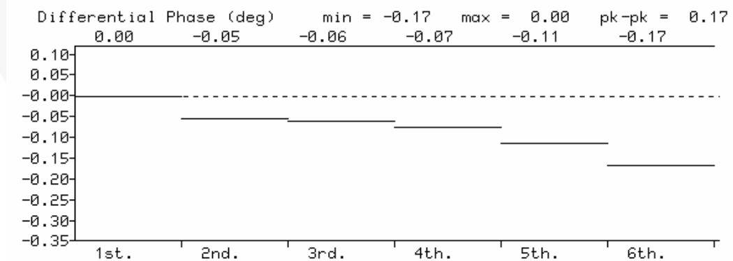
Figure 8. Differential Phase
