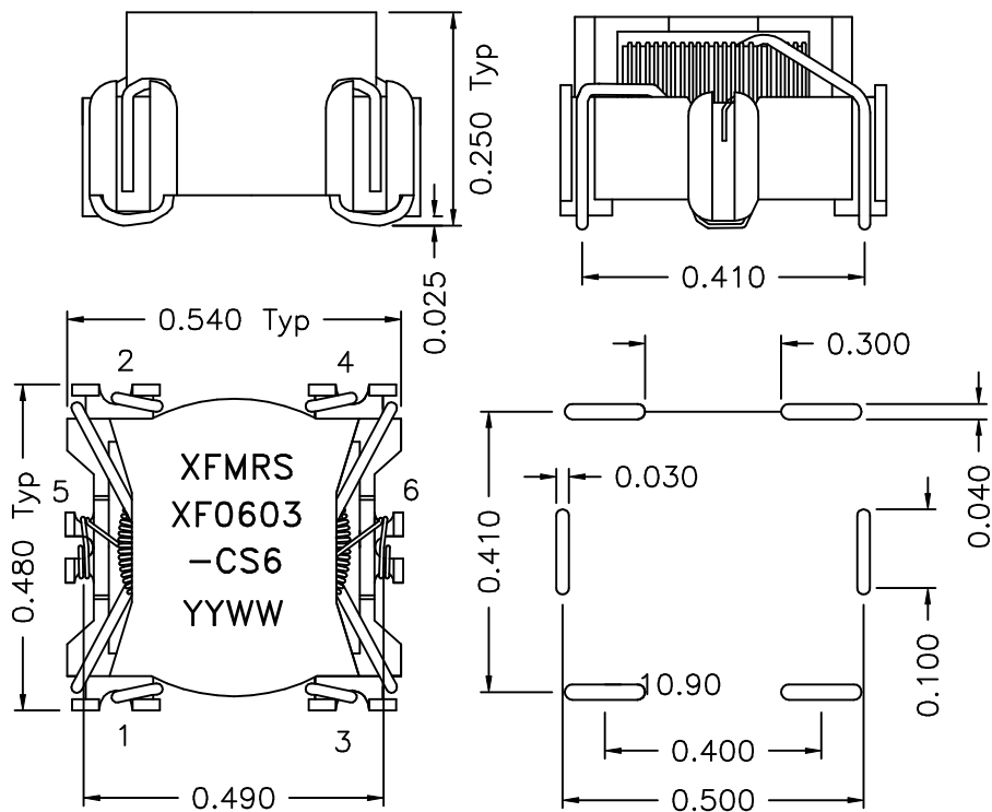
(SUGGESTED MOUNTING PAD)
