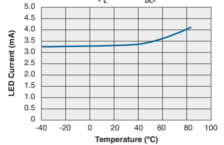
Typical I_F for Switch Operation vs. Temperature ( I_L=100mA_{DC} )
