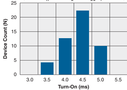
Typical Turn-On Time (N=50, T_A=25^\circ\text{C} , I_L=5\text{mA}_{DC} , I_F=10\text{mA} )
