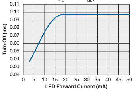
Typical Turn-Off vs. LED Forward Current ( I_L=100mA_{DC} )
