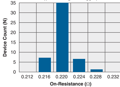
Typical On-Resistance Distribution (N=50, T_A=25^\circ\text{C} , I_L=1.0A_{DC} , I_F=10\text{mA} )
