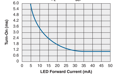
Typical Turn-On vs. LED Forward Current ( I_L=100\text{mA}_{DC} )
