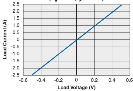
Typical Load Current vs. Load Voltage ( T_A=25°C, I_F=10mA )
