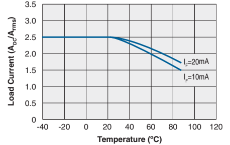
Typical Load Current vs. Temperature
