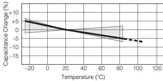
Char. E/Y5U ( Temp.Range:-25 to 85 °C max.Cap.Change:+20, -55 % )
