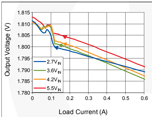
Figure 6. Voltage Regulation
