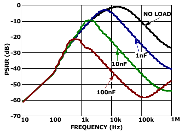
FIGURE 27. PSRR vs FREQUENCY
