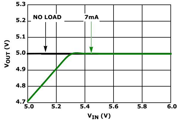
FIGURE 34. DROPOUT, ISL21080-50
