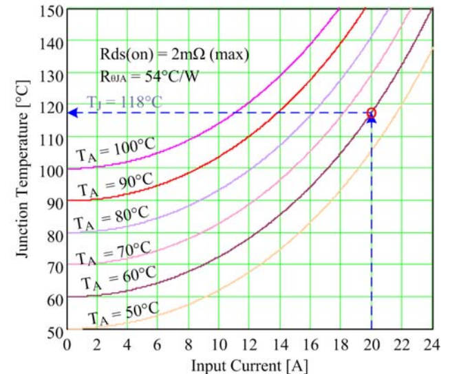
Figure 21: Example 1 final junction temperature at 20A/60°C T_A
