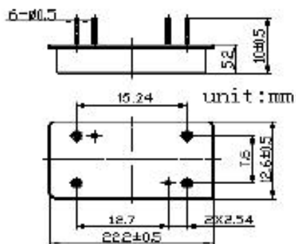
Package Outline
