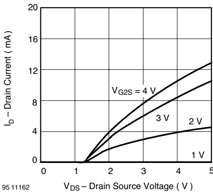
Figure 2. Drain Current vs. Drain Source Voltage
