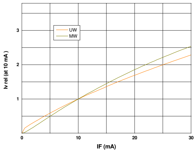
I_F - I_{v, \text{rel}} characteristic
