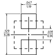
RECOMMENDED SMT LED SOLDER PATTERN SCALE: NTS
