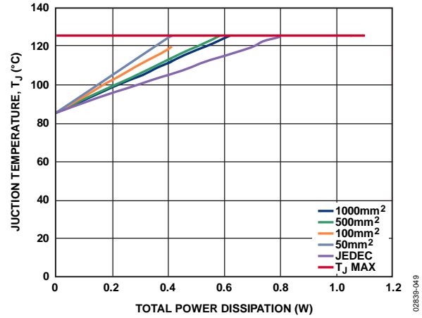
Figure 49. Junction Temperature vs. Total Power Dissipation, T_A = 85^\circ\text{C}
