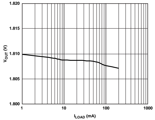
Figure 7. Output Voltage vs. Load Current
