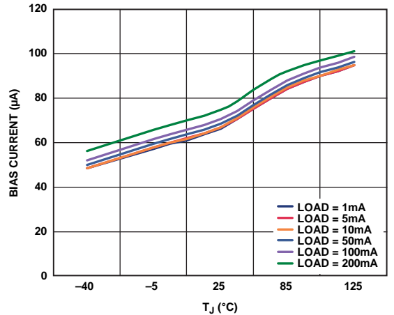
Figure 18. Bias Current vs. Junction Temperature, Single Output Loaded
