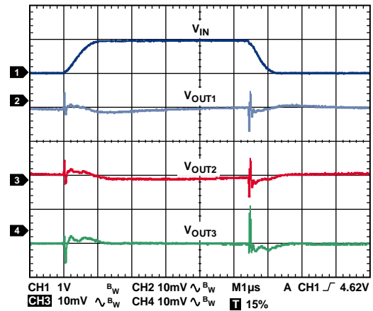
Figure 38. Line Transient Response, V_{IN} = 4V to 5V , I_{LOAD1} = I_{LOAD2} = I_{LOAD3} = 100mA , CH1 = V_{IN} , CH2 = V_{OUT1} , CH3 = V_{OUT2} , CH4 = V_{OUT3}
