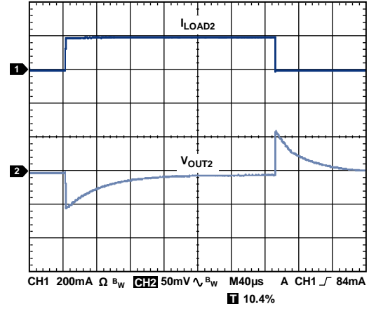
Figure 36. Load Transient Response, I_{LOAD2} = 1mA to 200mA , C_{OUT2} = 1\mu F , CH1 = I_{LOAD2} , CH2 = V_{OUT2}
