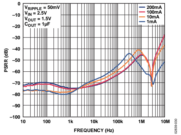
Figure 30. Power Supply Rejection Ratio vs. Frequency, 1.5 V
