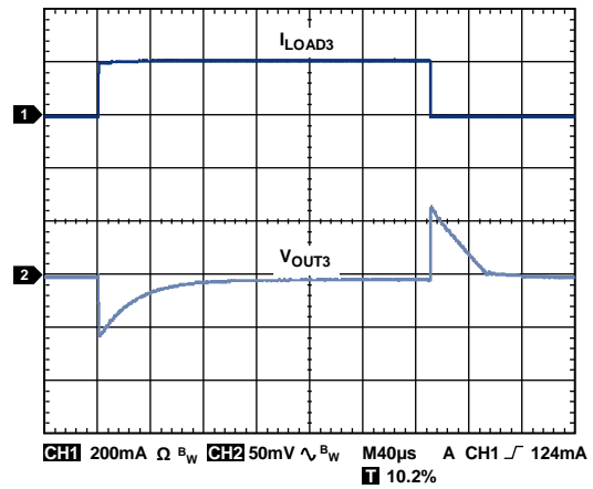
Figure 37. Load Transient Response, I_{LOAD3} = 1mA to 200mA , C_{OUT3} = 1\mu F , CH1 = I_{LOAD3} , CH2 = V_{OUT3}
