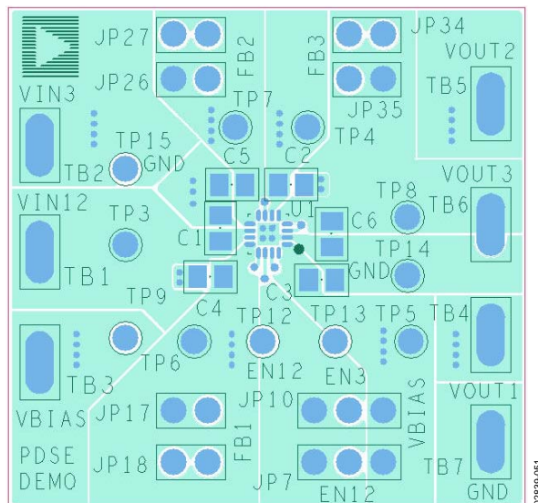
Figure 51. Example of PCB Layout, Top Side
