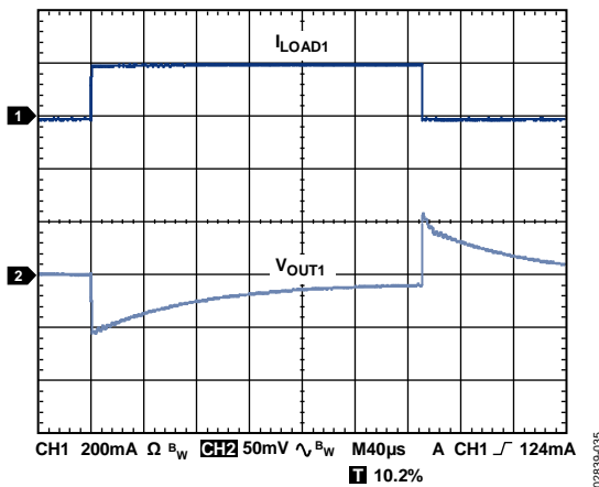
Figure 35. Load Transient Response, I_{LOAD1} = 1mA to 200mA , C_{OUT1} = 1\mu F , CH1 = I_{LOAD1} , CH2 = V_{OUT1}
