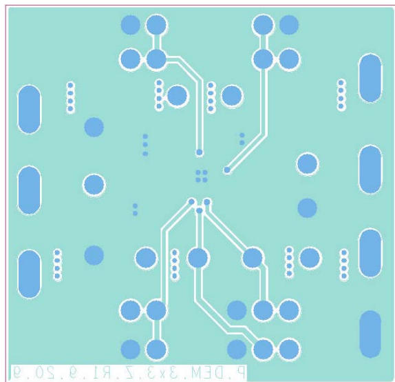
Figure 52. Example of PCB Layout, Bottom Side
