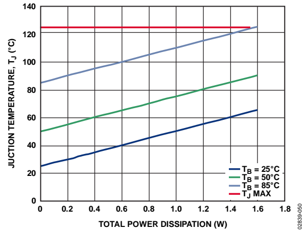
Figure 50. Junction Temperature vs. Total Power Dissipation and Board Temperature
