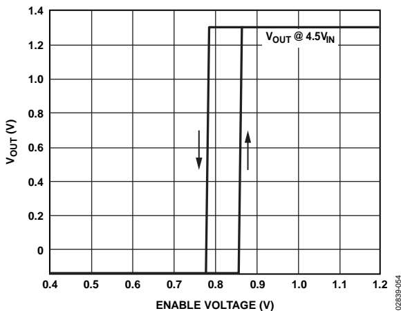
Figure 44. Typical EN_x Pin Operation
