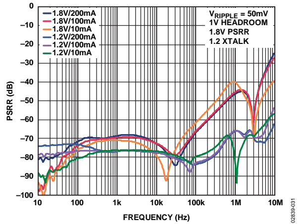
Figure 31. Power Supply Rejection Ratio vs. Frequency, Channel to Channel Crosstalk
