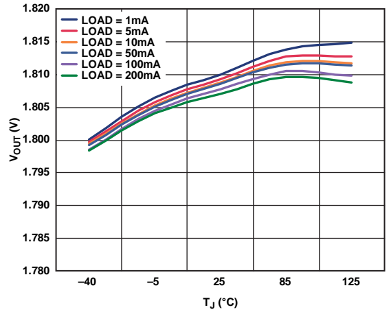
Figure 6. Output Voltage vs. Junction Temperature
