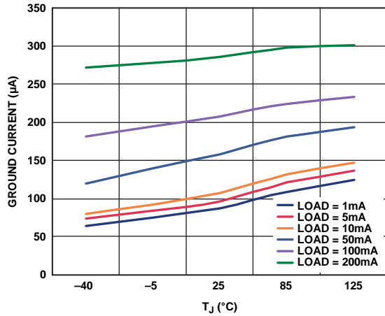
Figure 15. Ground Current vs. Junction Temperature, All Outputs Loaded Equally
