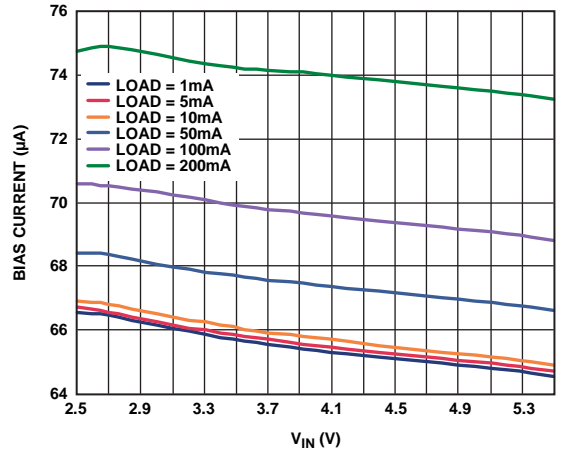
Figure 20. Bias Current vs. Input Voltage, Single Output Load
