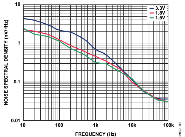
Figure 32. Output Noise Spectral Density, V_{IN} = 5\text{ V} , I_{LOAD} = 10\text{ mA}
