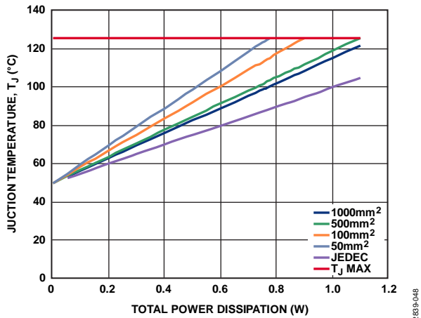
Figure 48. Junction Temperature vs. Total Power Dissipation, T_A = 50^\circ\text{C}
