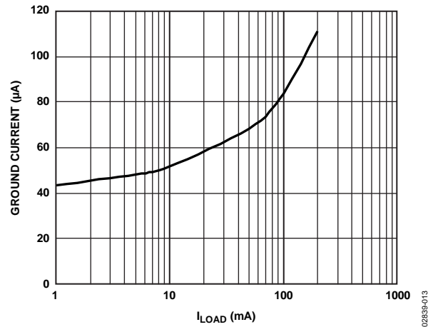
Figure 13. Ground Current vs. Load Current, Single Output Loaded
