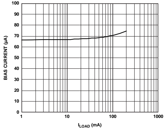
Figure 19. Bias Current vs. Load Current, Single Output Load
