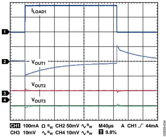
Figure 34. Load Transient Response, I_{LOAD1} = 1mA to 200mA , I_{LOAD2} = I_{LOAD3} = 1mA , CH1 = I_{LOAD1} , CH2 = V_{OUT1} , CH3 = V_{OUT2} , CH4 = V_{OUT3}
