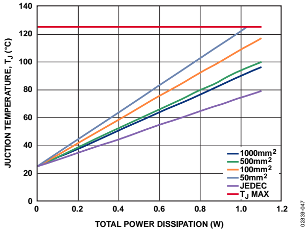
Figure 47. Junction Temperature vs. Total Power Dissipation, T_A = 25^\circ\text{C}
