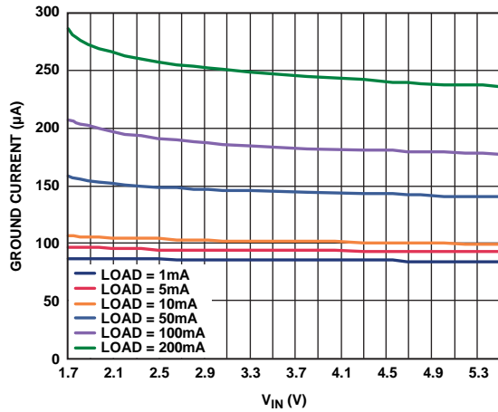
Figure 17. Ground Current vs. Input Voltage, All Outputs Loaded Equally
