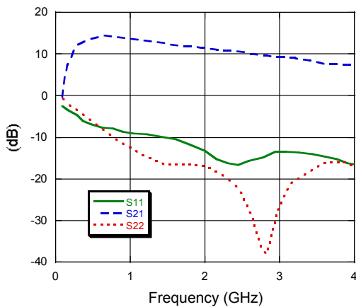
S-Parameters V_{DD} @ 5.0 V, T = 70\text{ }^\circ\text{C}
