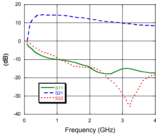
S-Parameters V_{DD} @ 5.0 V, T = -40\text{ }^\circ\text{C}
