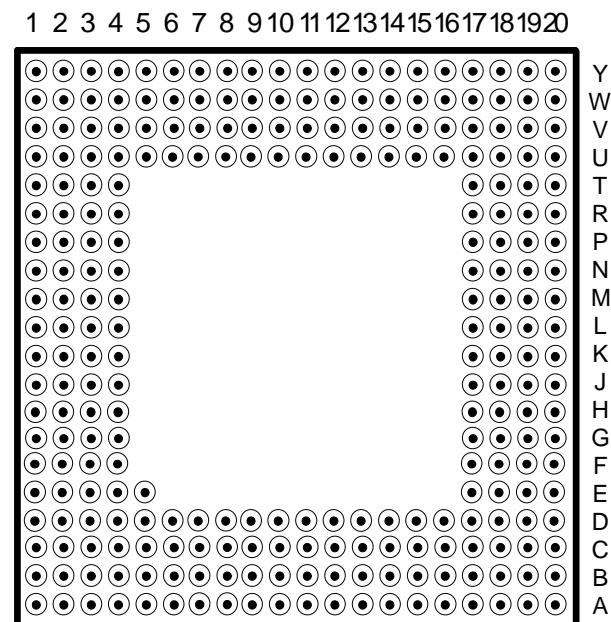
256-Pin CPGA
