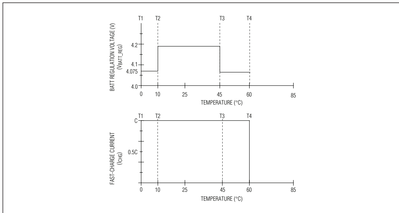
Figure 6. Safety Region 2: Fast-Charge Currents and Charge Termination Voltages
