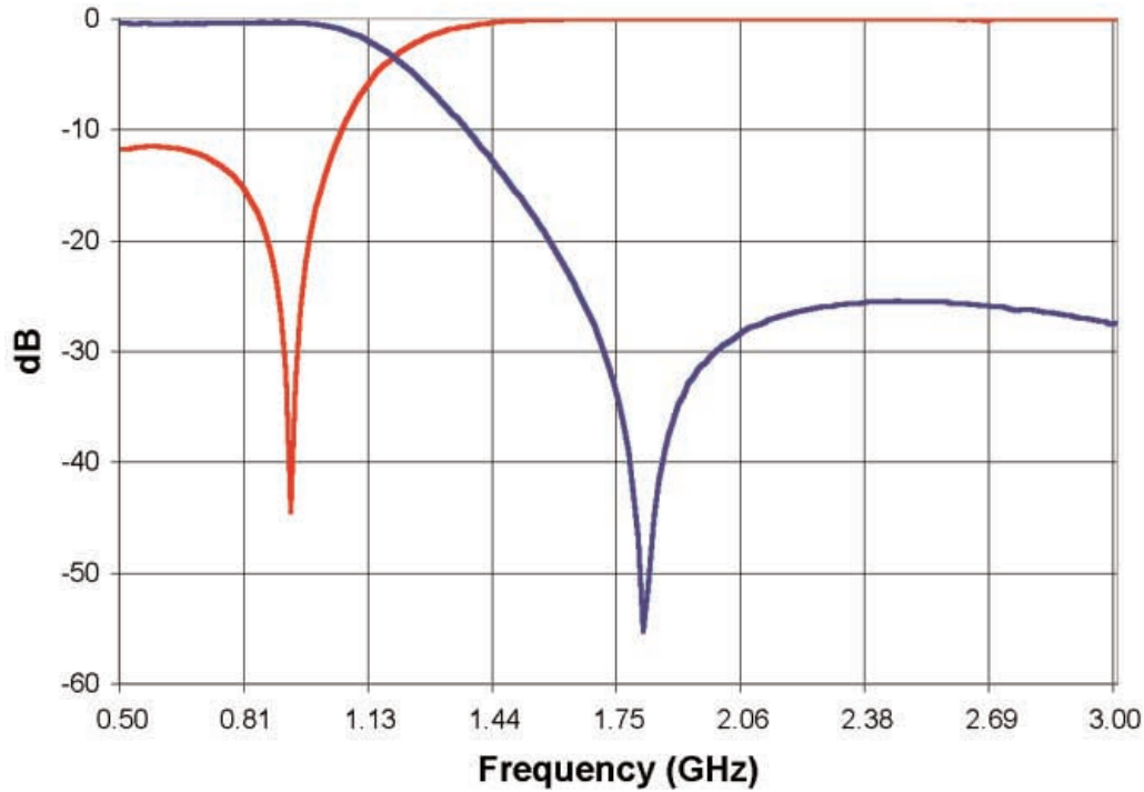
P/N 0898LP18A035 Low Pass Filter Typical Insertion Loss & Return Loss
