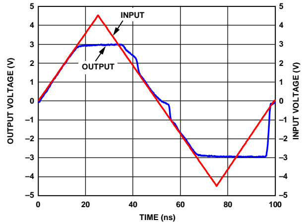
Figure 44. ADV3219 Overdrive Recovery
