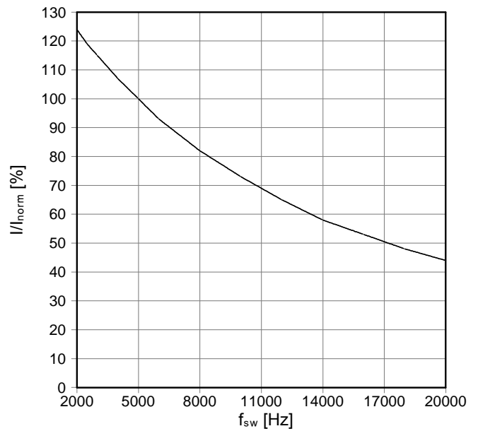
fsw - derating curves IGBT (motor) \cos(\phi) = 0,85 T_{cool\ medium} = 40^{\circ}C
