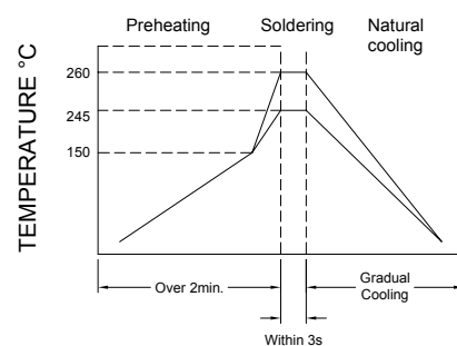
Figure 2. Wave Soldering
