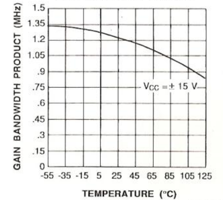
GAIN BANDWIDTH PRODUCT
