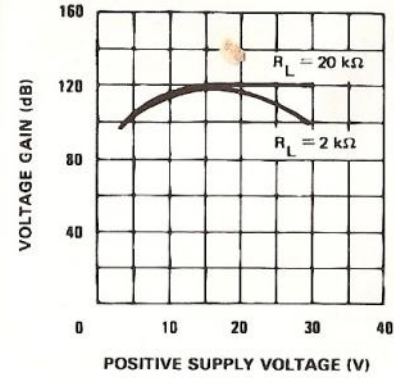
VOLTAGE GAIN
