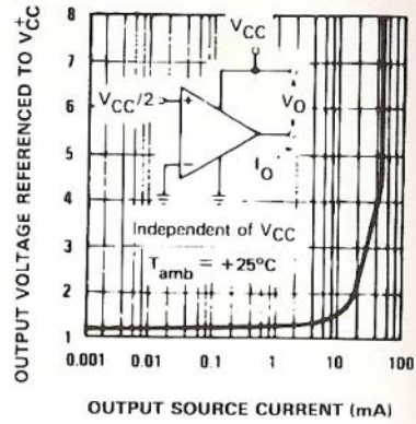
OUTPUT CHARACTERISTICS
