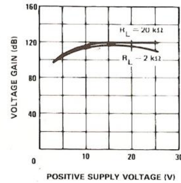
VOLTAGE GAIN
