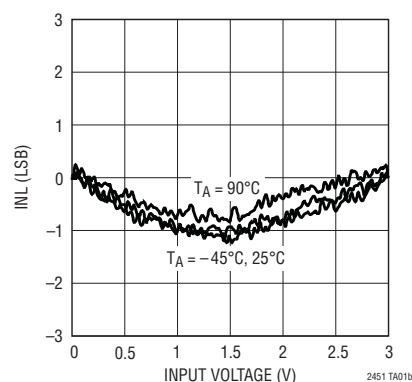
Integral Nonlinearity, V CC = 3V
