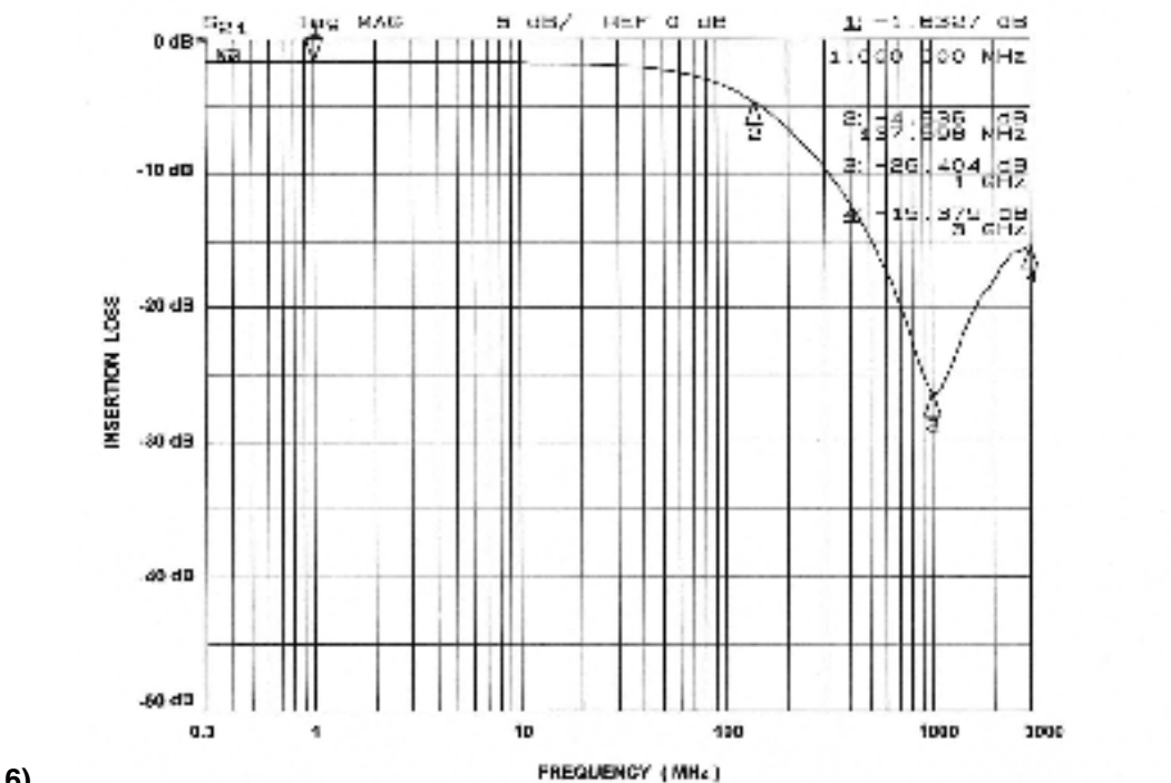
6) Figure 4. Insertion Loss vs. Frequency Performance Curve, PACUSBVBD3 (SOT23-6)
