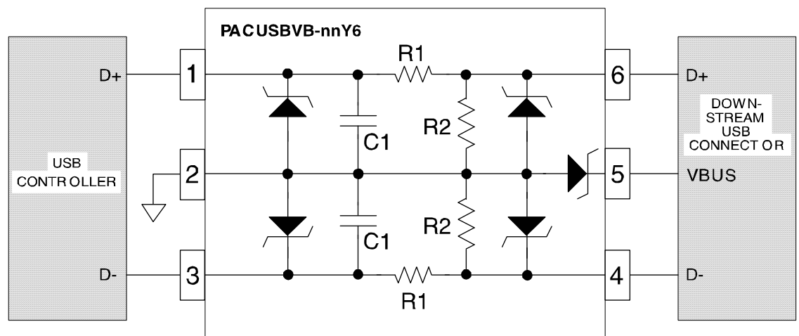
Connection Diagram for PACUSBVB-D1/D2/D3
