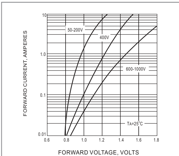
Fig.3 FORWARD CHARACTERISTICS
