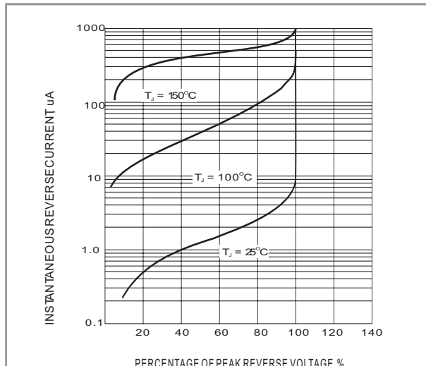
Fig.4-TYPICAL REVERSE CHARACTERISTIC
