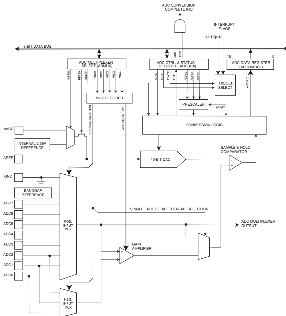
Figure 23-1. Analog to Digital Converter Block Schematic
