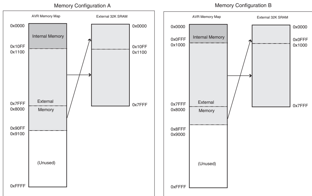
Figure 7-10. Address Map with 32 KB External Memory
