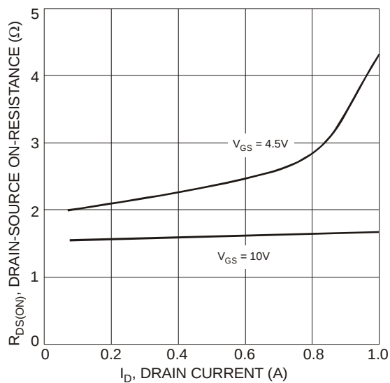
Fig. 4 On Resistance vs. Drain Current
