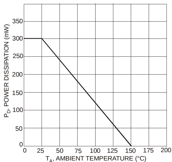
Fig. 6 Max Power Dissipation vs. Ambient Temperature
