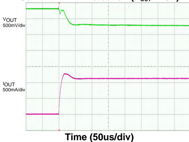
Short Circuit Protection (V OUT =1.8V)
