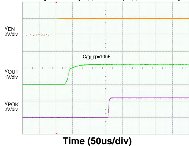
Start-up Time ( V_{OUT} = 1.2V , I_{OUT} = 600mA )
