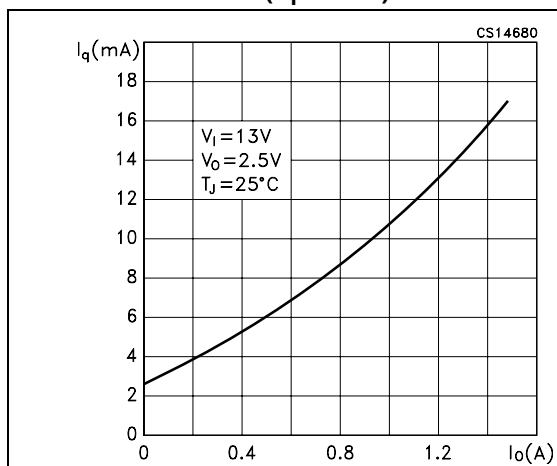
Figure 9. Quiescent current vs. output current ( V_I = 13V )
