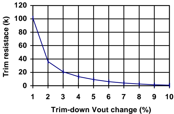
Fig 5 Trim-down output vs. trim resistance
