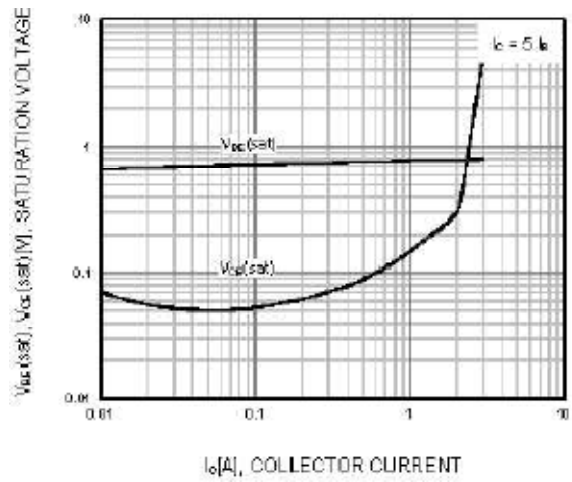
Fig. 2 Saturation Voltage
