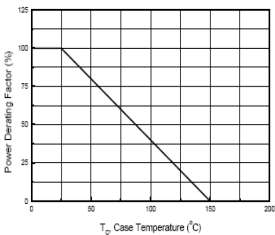
Fig. 5 Power Derating
