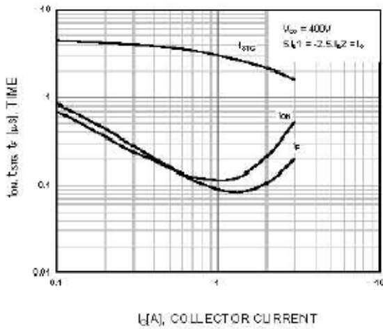
Fig. 3 Switching Time
