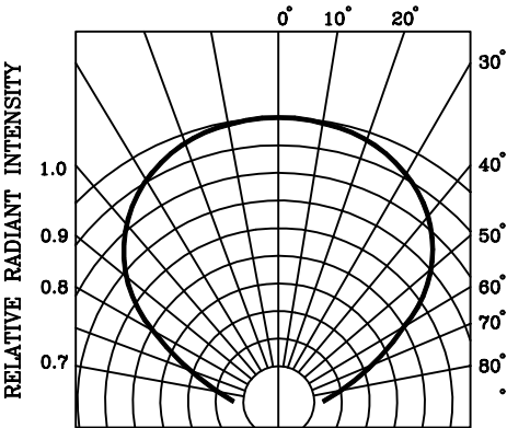
Fig.6 RADIATION DIAGRAM
