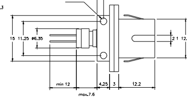
SC Receptacle (Board Mount)
