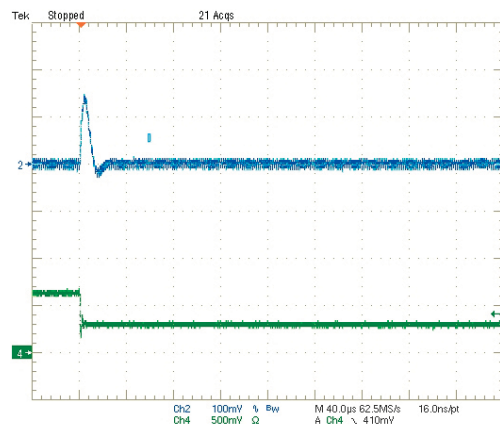
Step Load Transient Response (Vin=5V, Vout=1.5V, Clod=0, Iout=3A to 1.5A) Trace 2=Vout, 100 mV/div. Trace 4=Iout, 1A/div.
