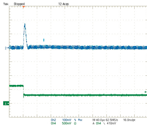
Step Load Transient Response (Vin=5V, Vout=3.3V, Cload=0, Iout=3A to 1.5A) Trace 2=Vout, 100 mV/div. Trace 4=Iout, 1A/div.
