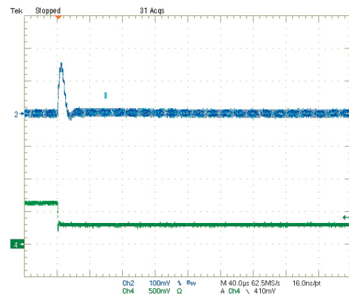
Step Load Transient Response (Vin=5V, Vout=2.5V, Cload=0, Iout=3A to 1.5A) Trace 2=Vout, 100 mV/div. Trace 4=Iout, 1A/div.
