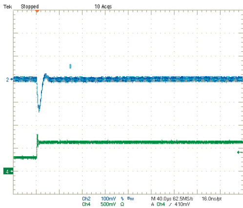
Step Load Transient Response (Vin=5V, Vout=1.8V, Load=0, Iout=1.5A to 3A) Trace 2=Vout, 100 mV/div. Trace 4=Iout, 1A/div.
