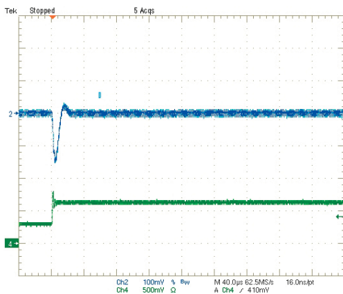
Step Load Transient Response (Vin=5V, Vout=1.5V, Clod=0, Iout=1.5A to 3A) Trace 2=Vout, 100 mV/div. Trace 4=Iout, 1A/div.
