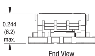
End View
