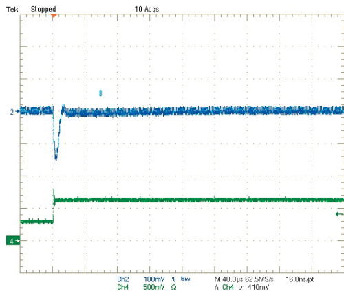
Step Load Transient Response (Vin=5V, Vout=3.3V, Cload=0, Iout=1.5A to 3A) Trace 2=Vout, 100 mV/div. Trace 4=Iout, 1A/div.
