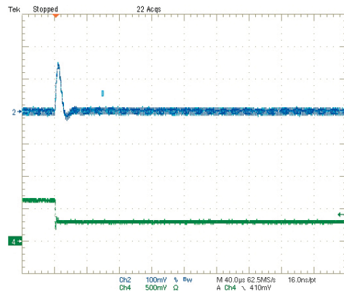
Step Load Transient Response (Vin=5V, Vout=1.8V, Load=0, Iout=3A to 1.5A) Trace 2=Vout, 100 mV/div. Trace 4=Iout, 1A/div.
