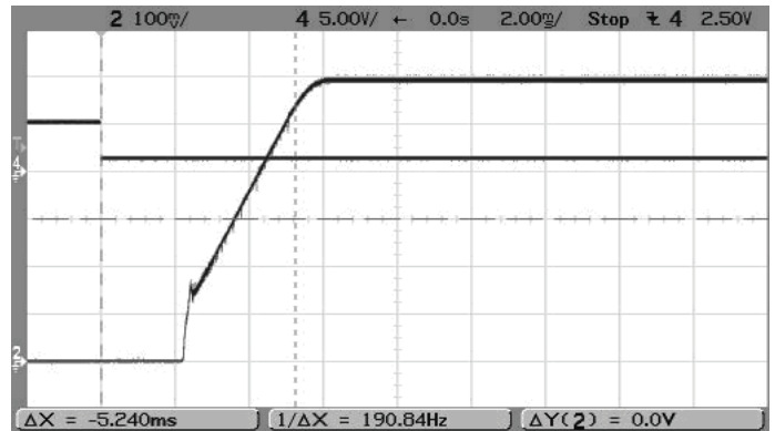
Step Load Transient Response (Vin=5V, Vout=0.6V, Load=0, Iout=3A to 1.5A) Trace 2=Vout, 100 mV/div. Trace 4=Iout, 1A/div.
