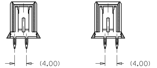
SECTION: Y-Y SECTION: W-W
