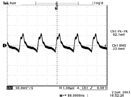
3.3 Vdc input, 15 Vdc output
