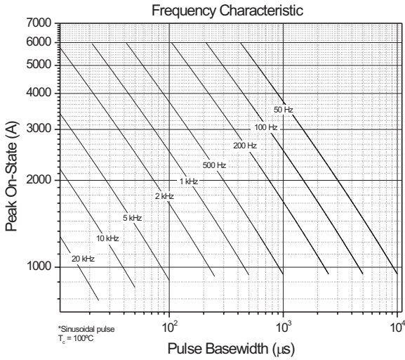
Fig. 11 - Frequency Characteristics
