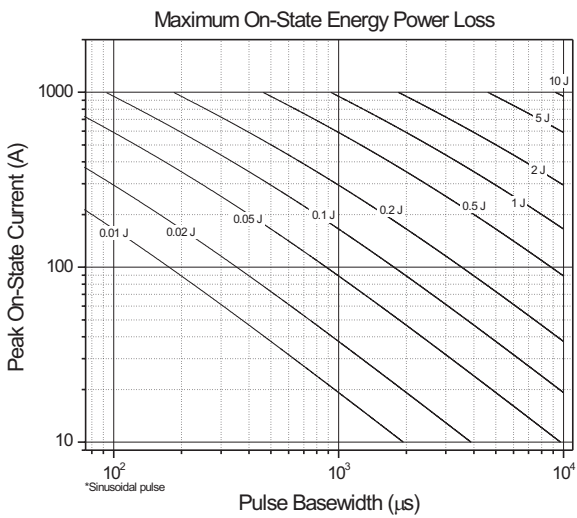
Fig. 13 - Maximum On-State Power Loss Characteristics
