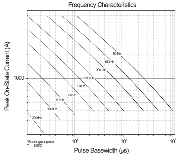
Fig. 12 - Frequency Characteristics
