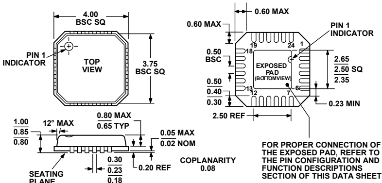
Figure 104. 24-Lead Lead Frame Chip Scale Package [LFCSP_VQ] 4 mm × 4 mm Body, Very Thin Quad (CP-24-3) Dimensions shown in millimeters
