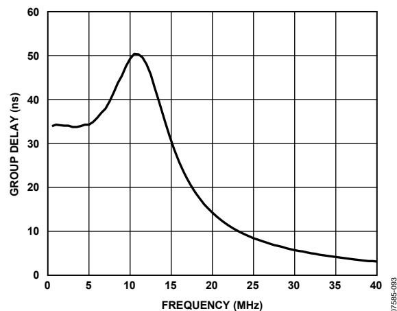
Figure 94. Fourth-Order Low-Pass LTE Filter Group Delay Response
