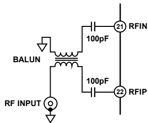
Figure 79. RF Input
