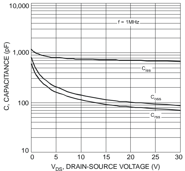
Fig. 8 Total Capacitance
